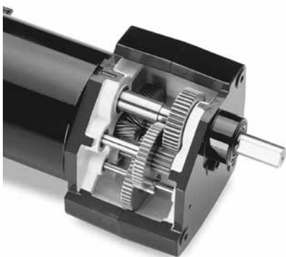
Combination of spur and helical gears can be seen in this cutaway view of a sub-fractional horsepower parallel-shaft gearbox. Note multiple gear stages.
